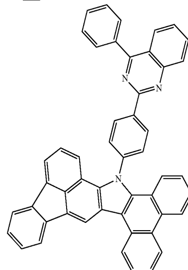
Compound 35
