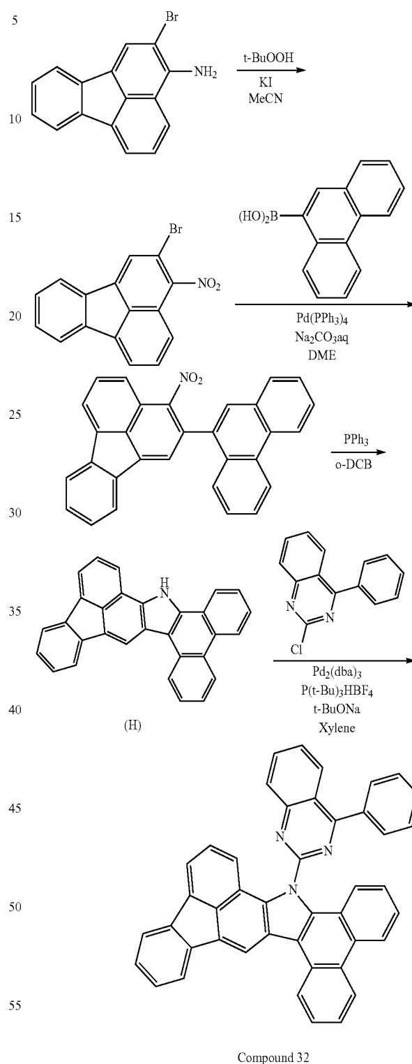
Compound 32
