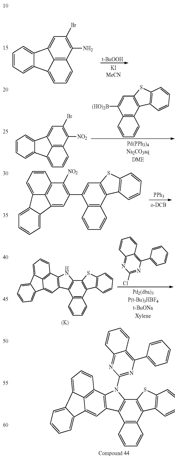
Compound 44
