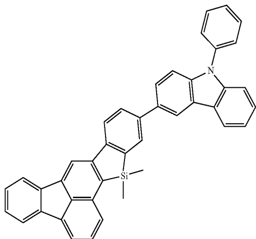
Compound 19
