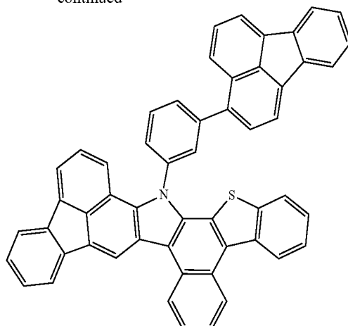
Compound 46
