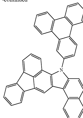
Compound 29
