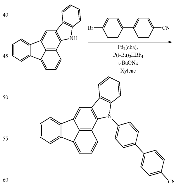
Compound 22
