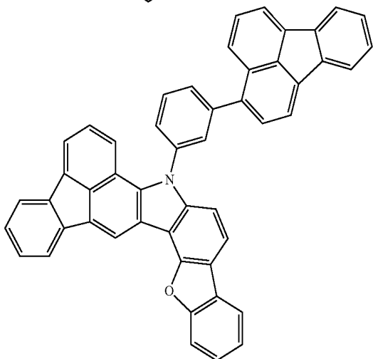
Compound 42
