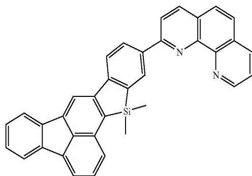
Compound 26
