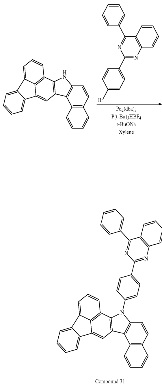
Compound 31
