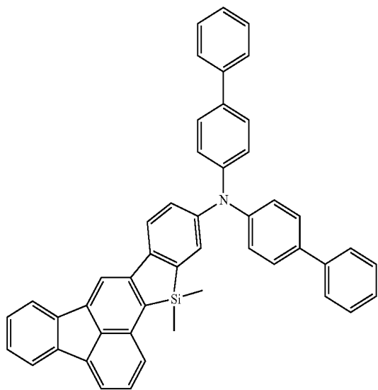
Compound 24
