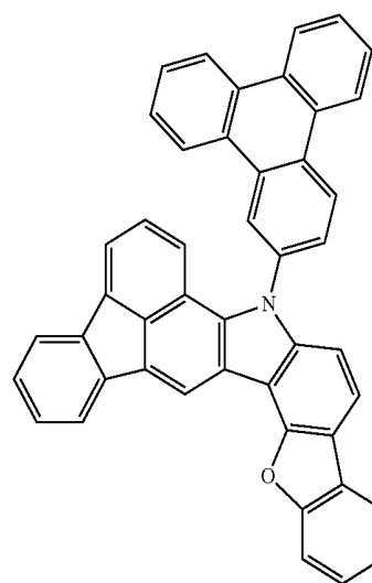
Compound 41
