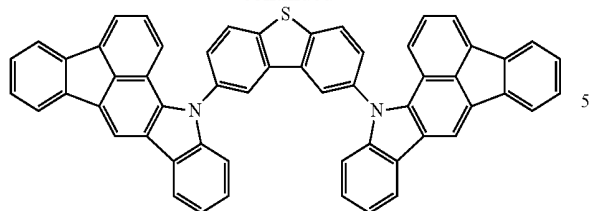
Compound 19
