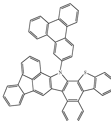
Compound 45
