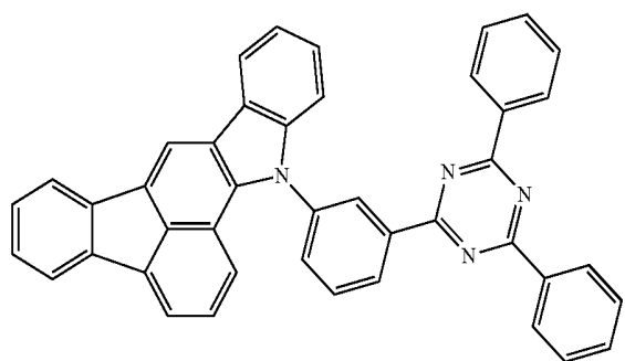
Comparative compound 1
