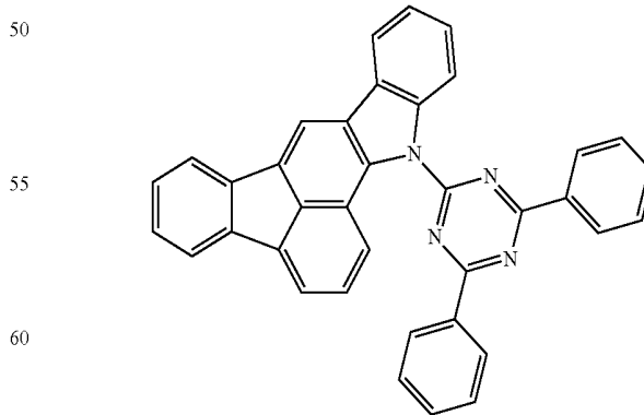
Compound 12
