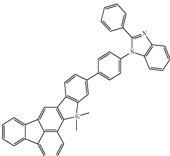
Compound 24
