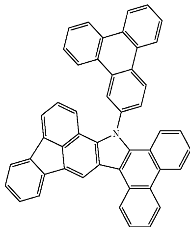
Compound 33
