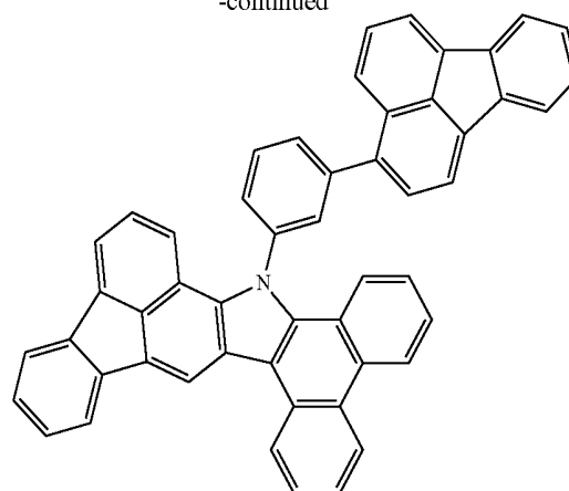
Compound 34
