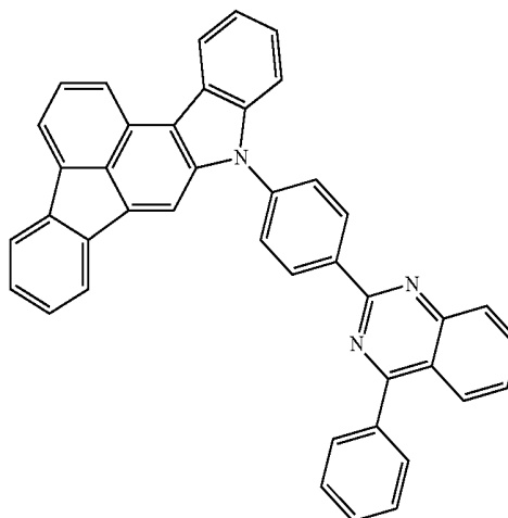
Comparative compound 2
