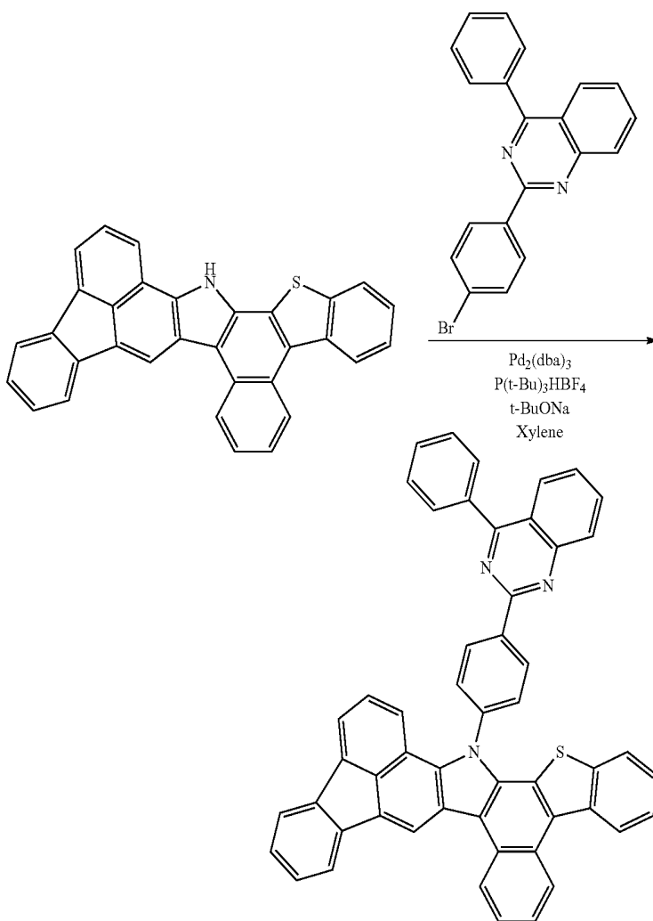
Compound 47
