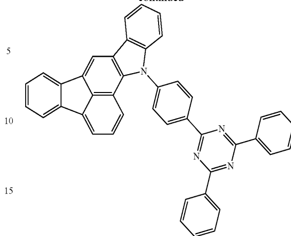
Compound 11
