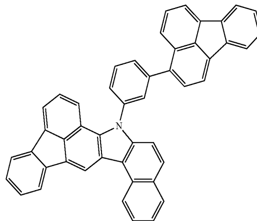
Compound 30
