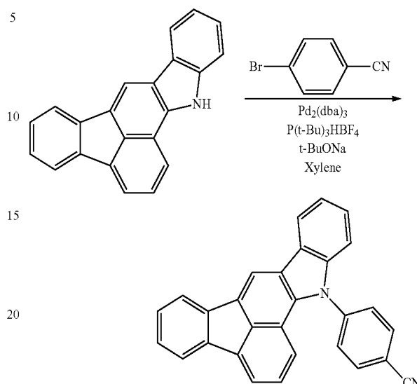
Compound 21
