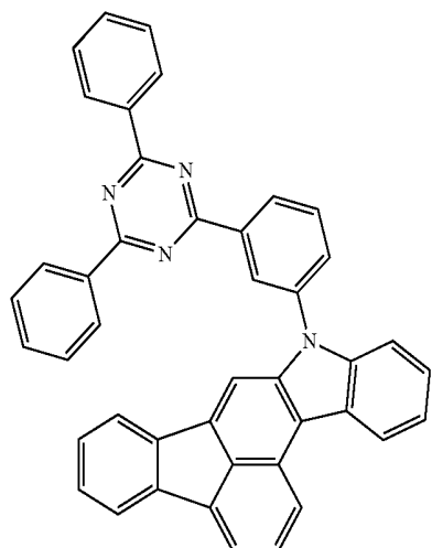
Comparative compound 1
