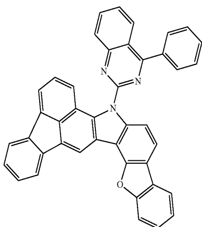
Compound 40
