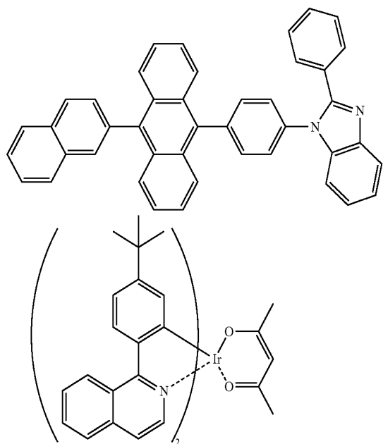
Compound 2
